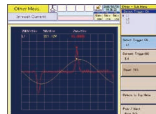
▲ Rush current measurement (KHA3000)
